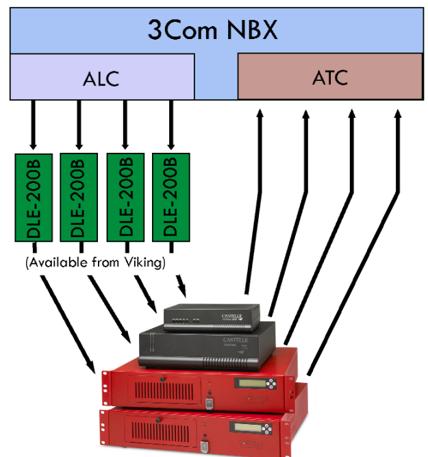
Integration of your FaxPress with 3Com's NBX PBX
